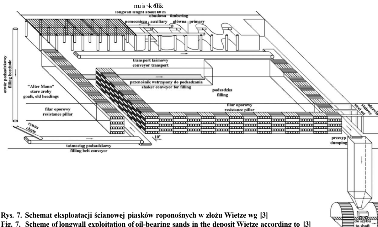
Fig. 7. Scheme of longwall exploitation of oil-bearing sands in the deposit Wietze according to [3]
